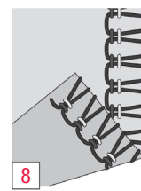
8 3-Faden-Overlock- Stretch
